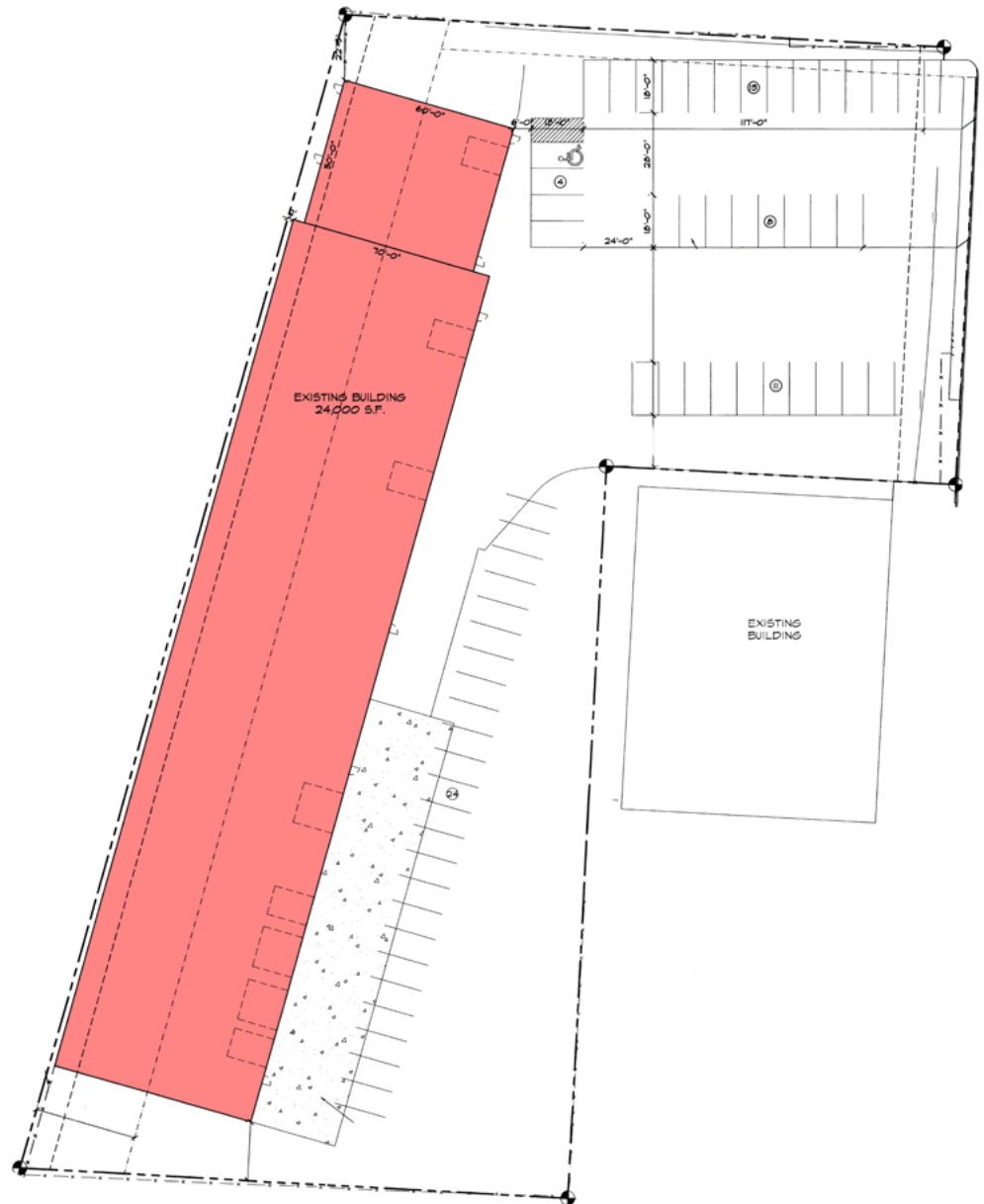
Site Plan
